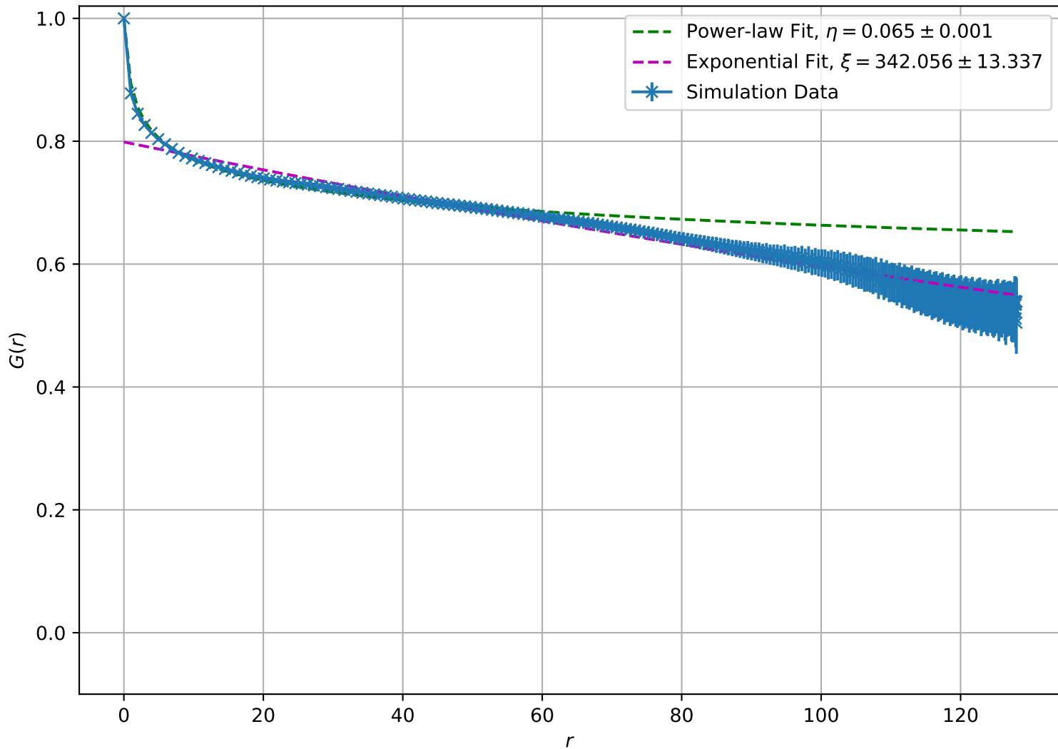
Correlation Function at T = 6.00\text{e} - 01 , L = 128
