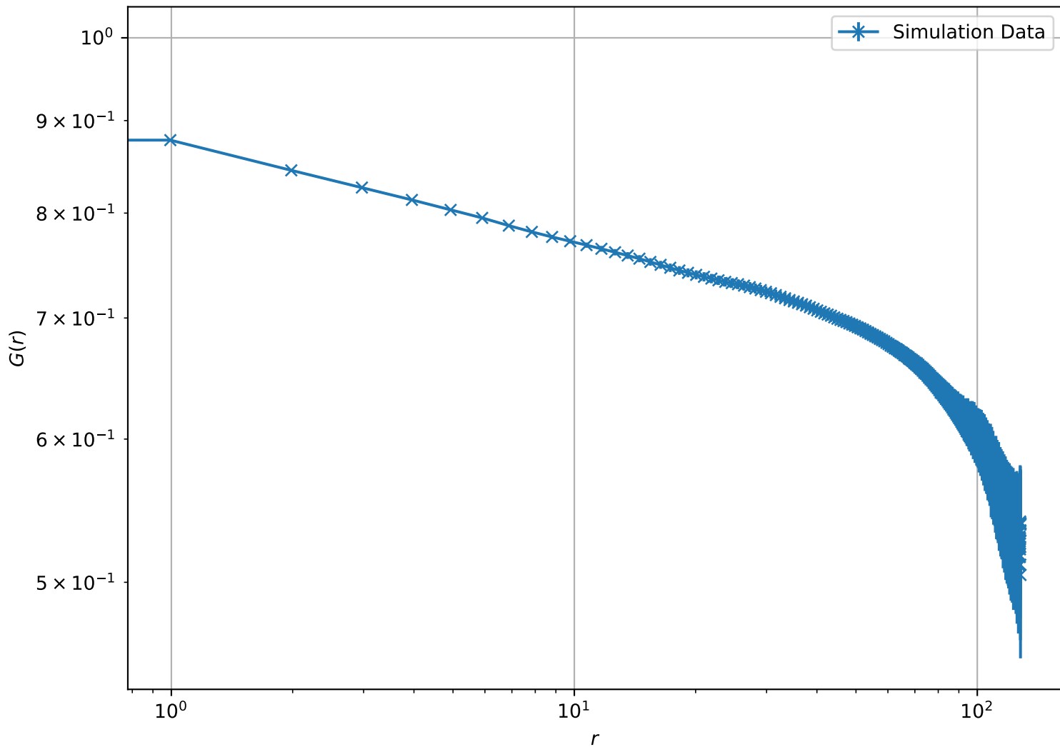
Correlation Function at T = 6.00e - 01 , L = 128 (Log-Log Scale)
