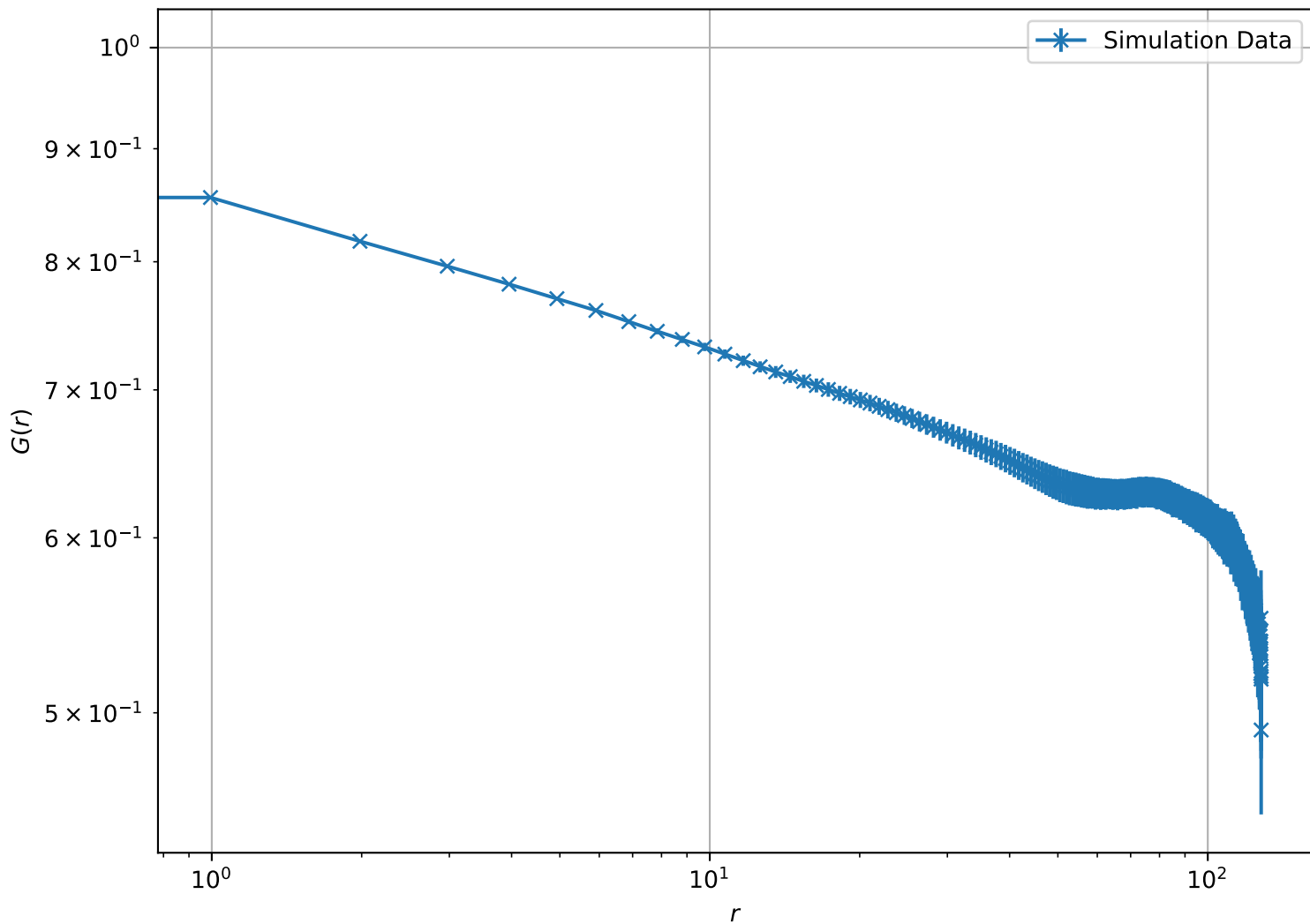
Correlation Function at T = 7.00e - 01 , L = 128 (Log-Log Scale)
