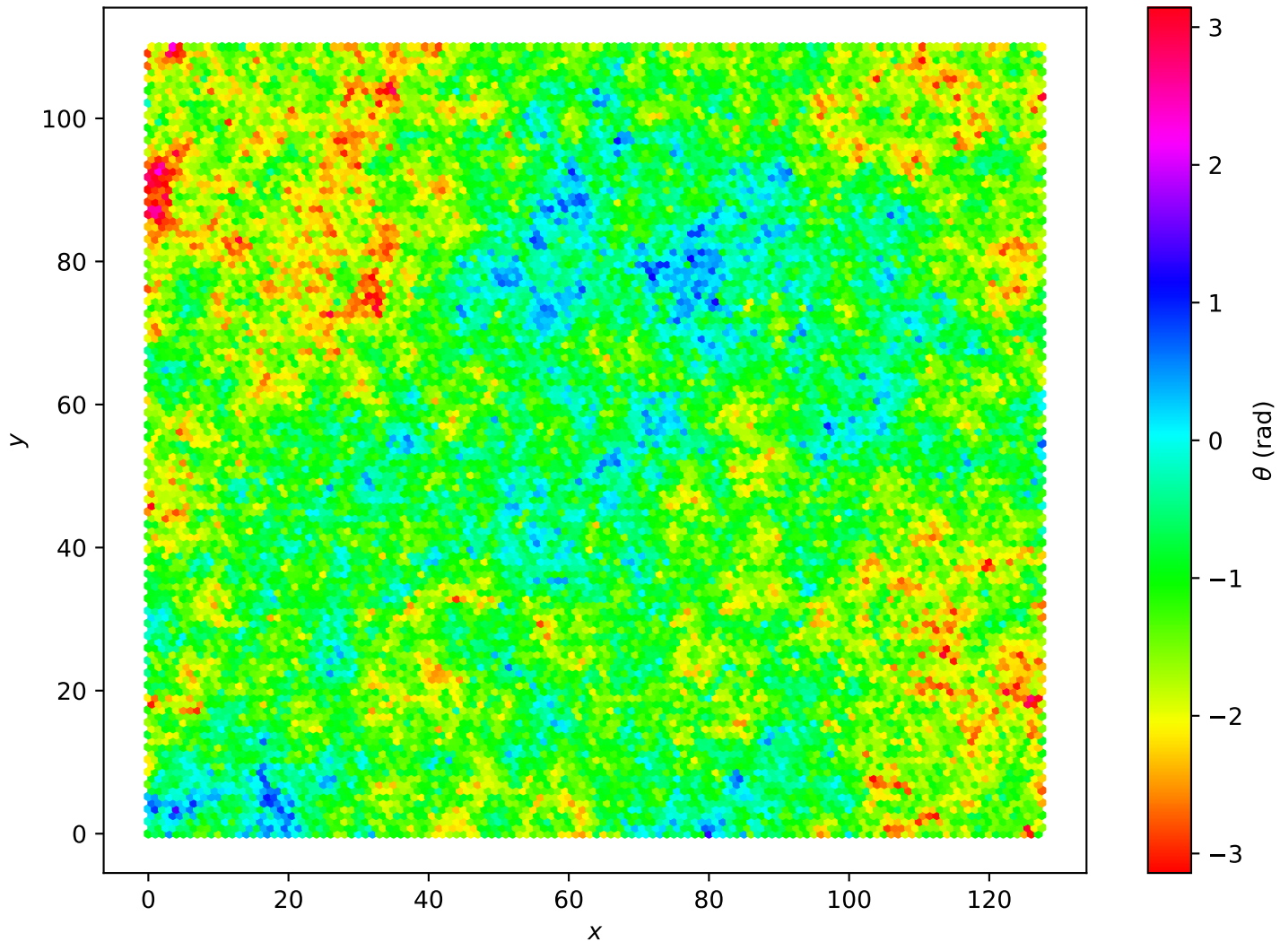
Hexagonal Lattice L=128 , T = 7.00e - 01
