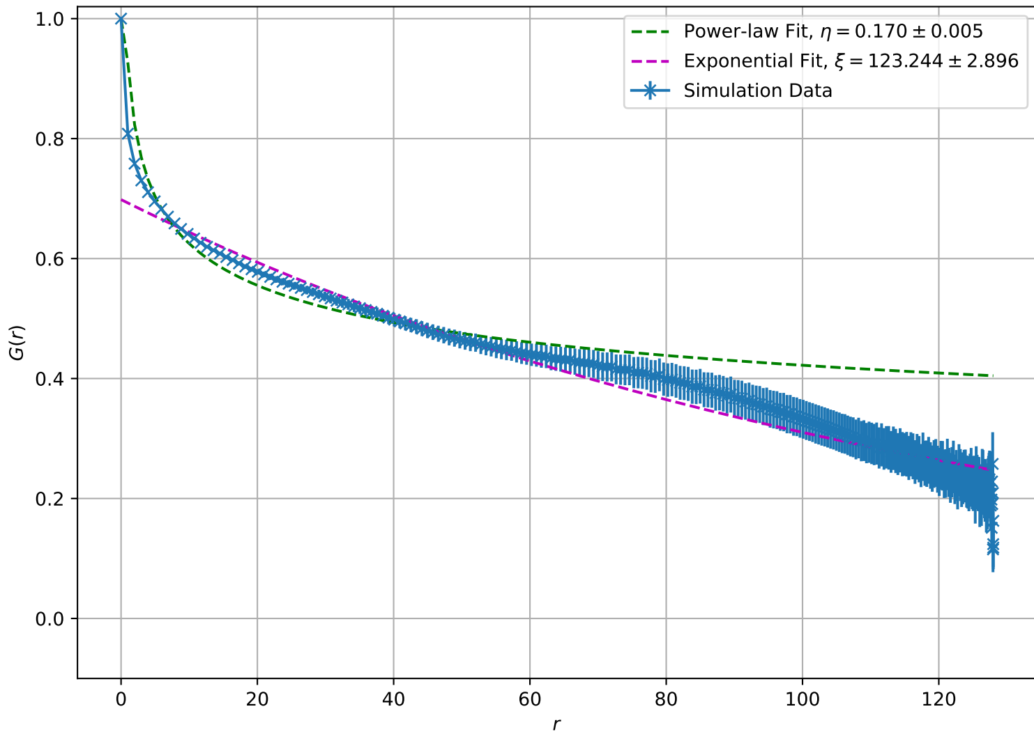
Correlation Function at T = 9.00e - 01 , L = 128
