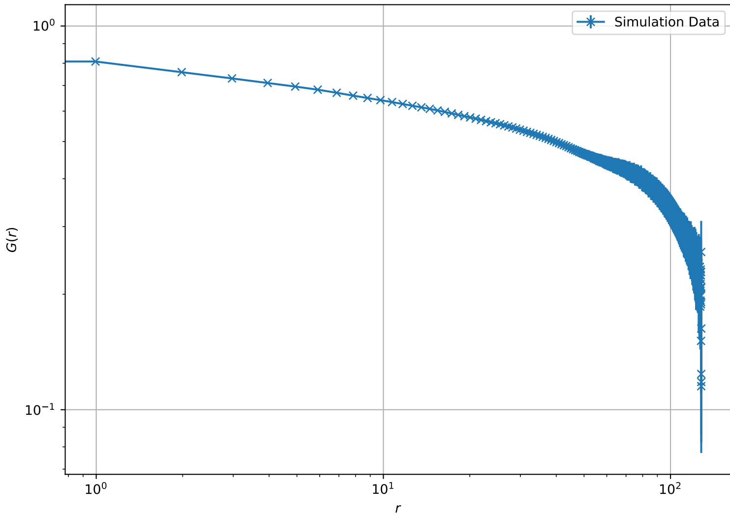
Correlation Function at T = 9.00e - 01 , L = 128 (Log-Log Scale)
