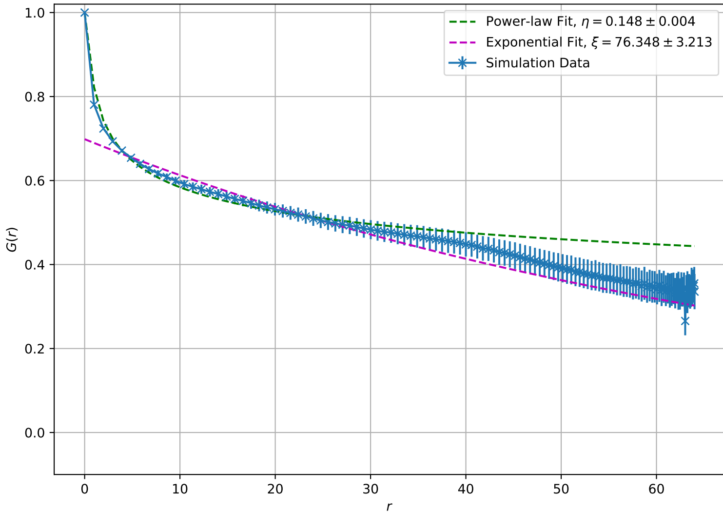
Correlation Function at T = 1.00\text{e} + 00 , L = 64
