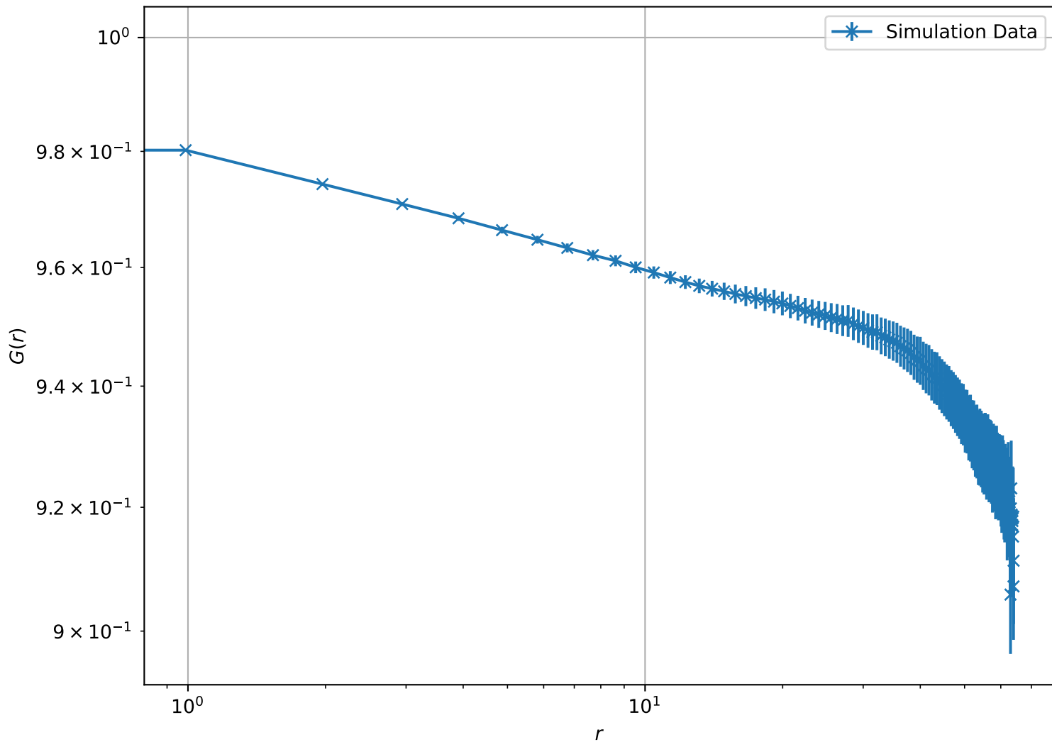
Correlation Function at T = 1.00e - 01 , L = 64 (Log-Log Scale)
