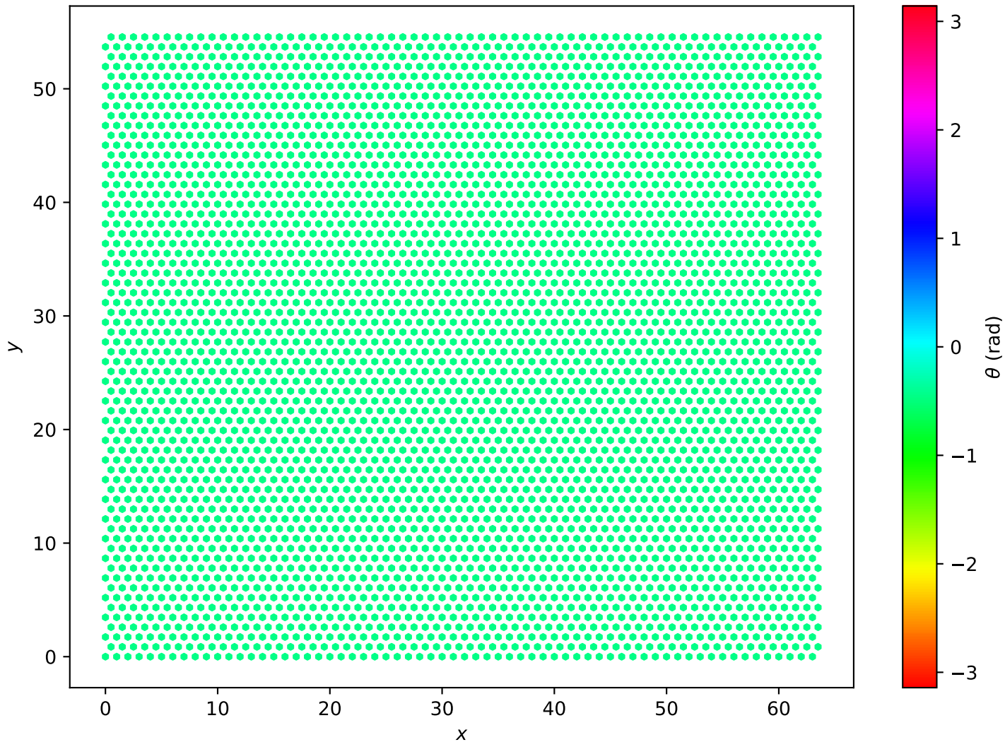
Hexagonal Lattice L=64 , T = 1.00e - 05
