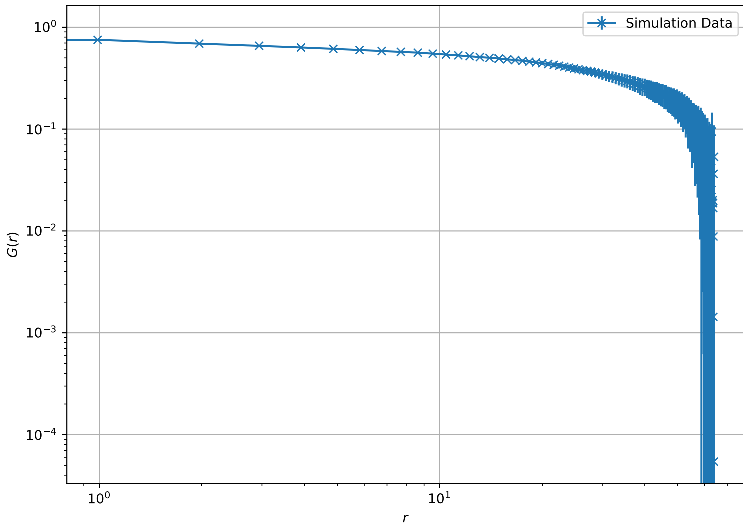
Correlation Function at T = 1.10e + 00 , L = 64 (Log-Log Scale)
