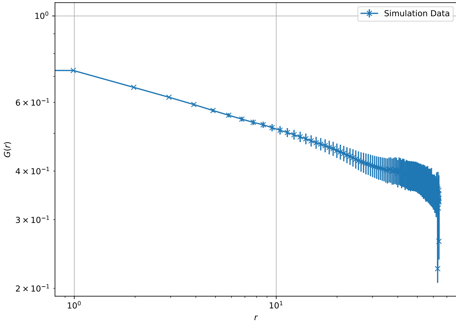
Correlation Function at T = 1.20e + 00 , L = 64 (Log-Log Scale)
