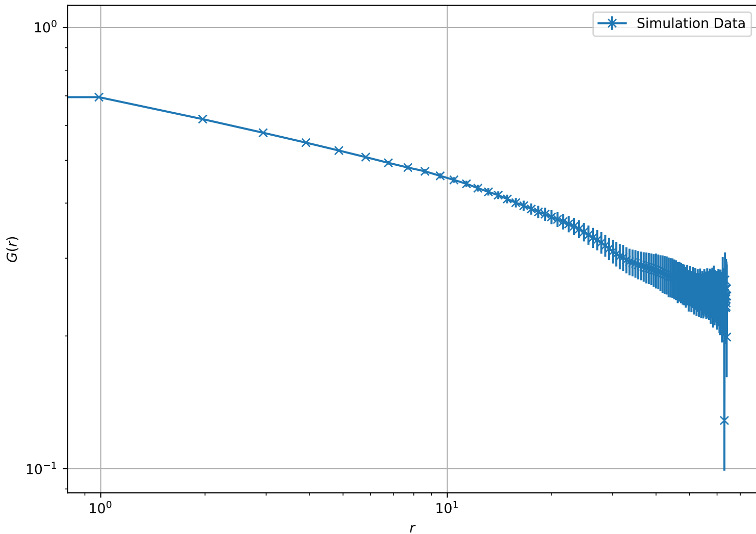
Correlation Function at T = 1.30e + 00 , L = 64 (Log-Log Scale)
