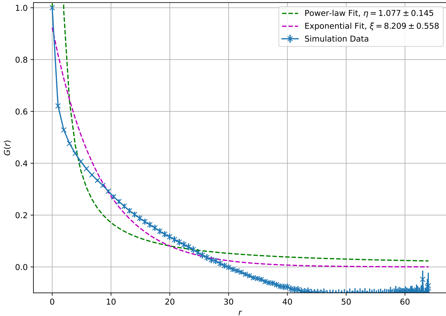
Correlation Function at T = 1.50e + 00 , L = 64
