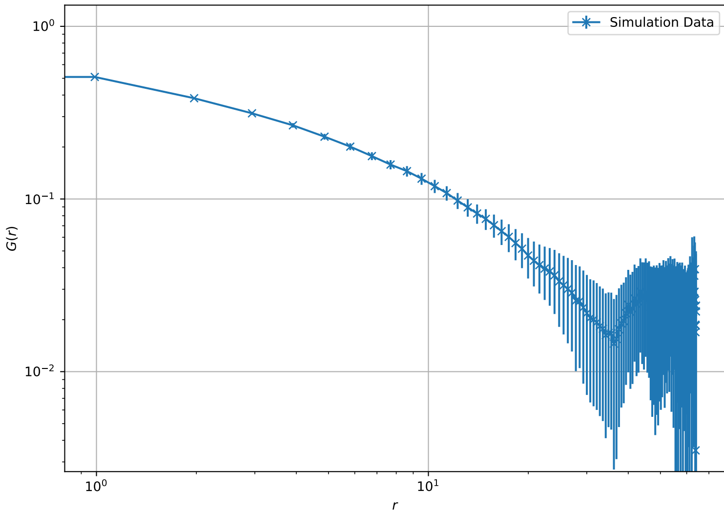
Correlation Function at T = 1.70e + 00 , L = 64 (Log-Log Scale)
