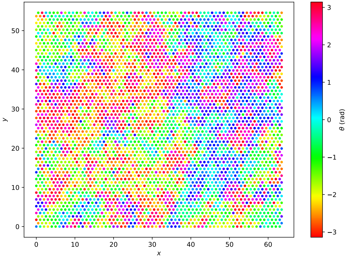
Hexagonal Lattice L=64 , T = 1.70e + 00
