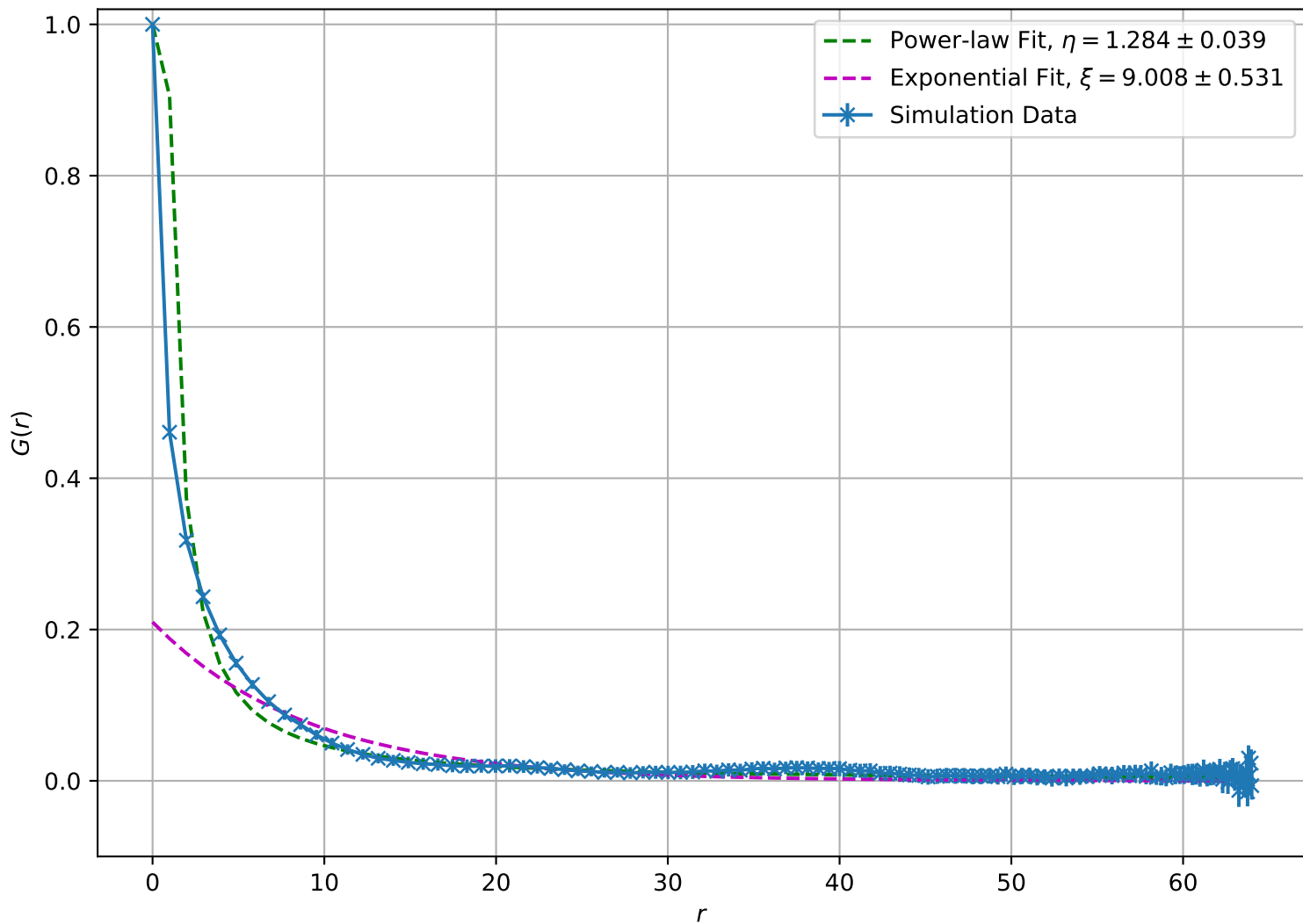
Correlation Function at T = 1.80e + 00 , L = 64
