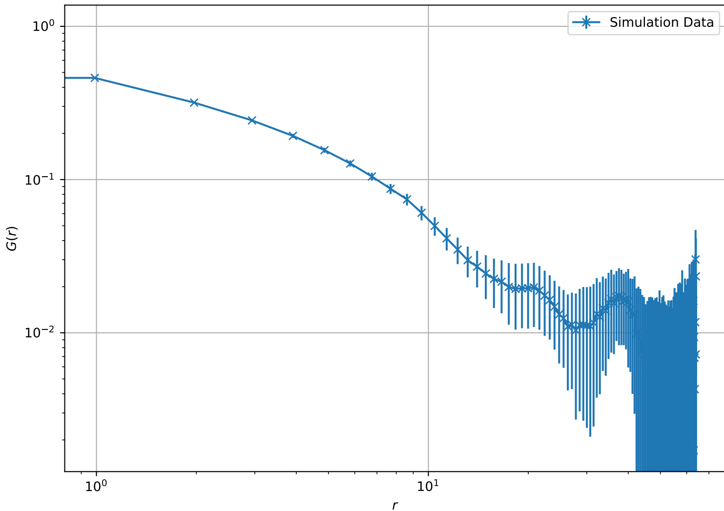
Correlation Function at T = 1.80e + 00 , L = 64 (Log-Log Scale)
