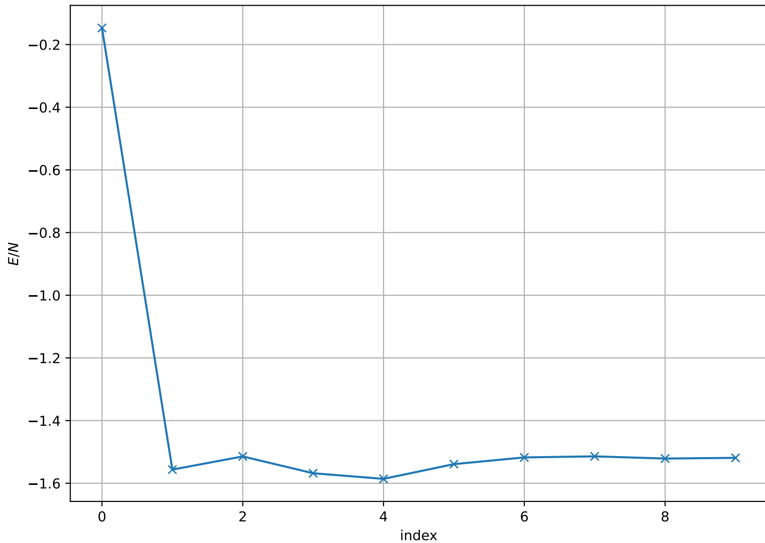
Energy per Site at T = 1.800e + 00 , L = 64
