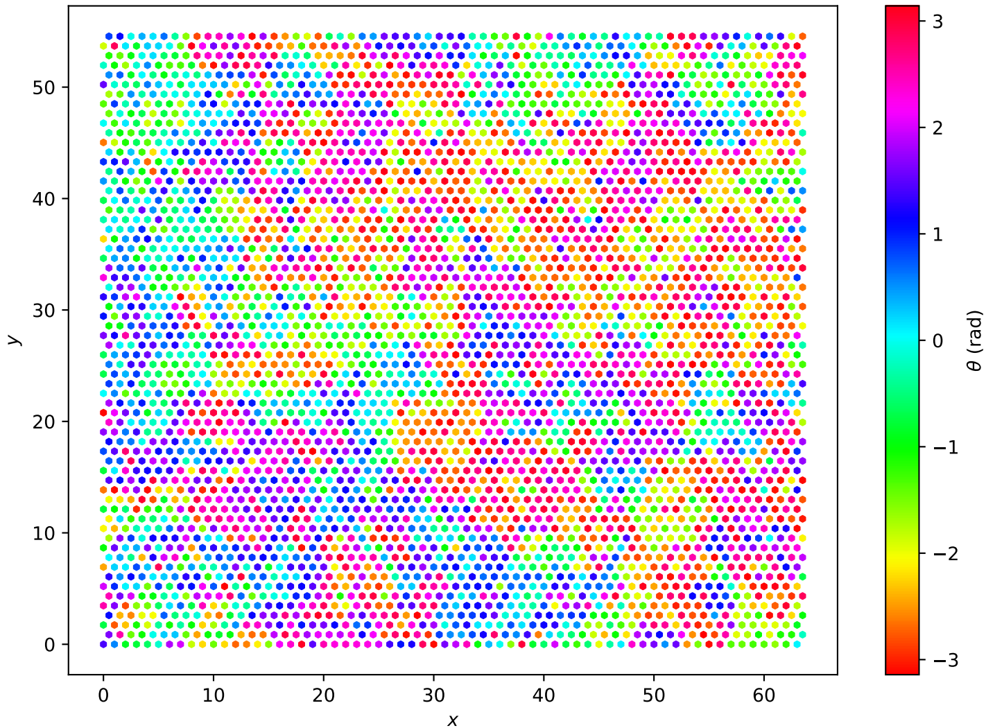
Hexagonal Lattice L=64 , T = 1.90e + 00
