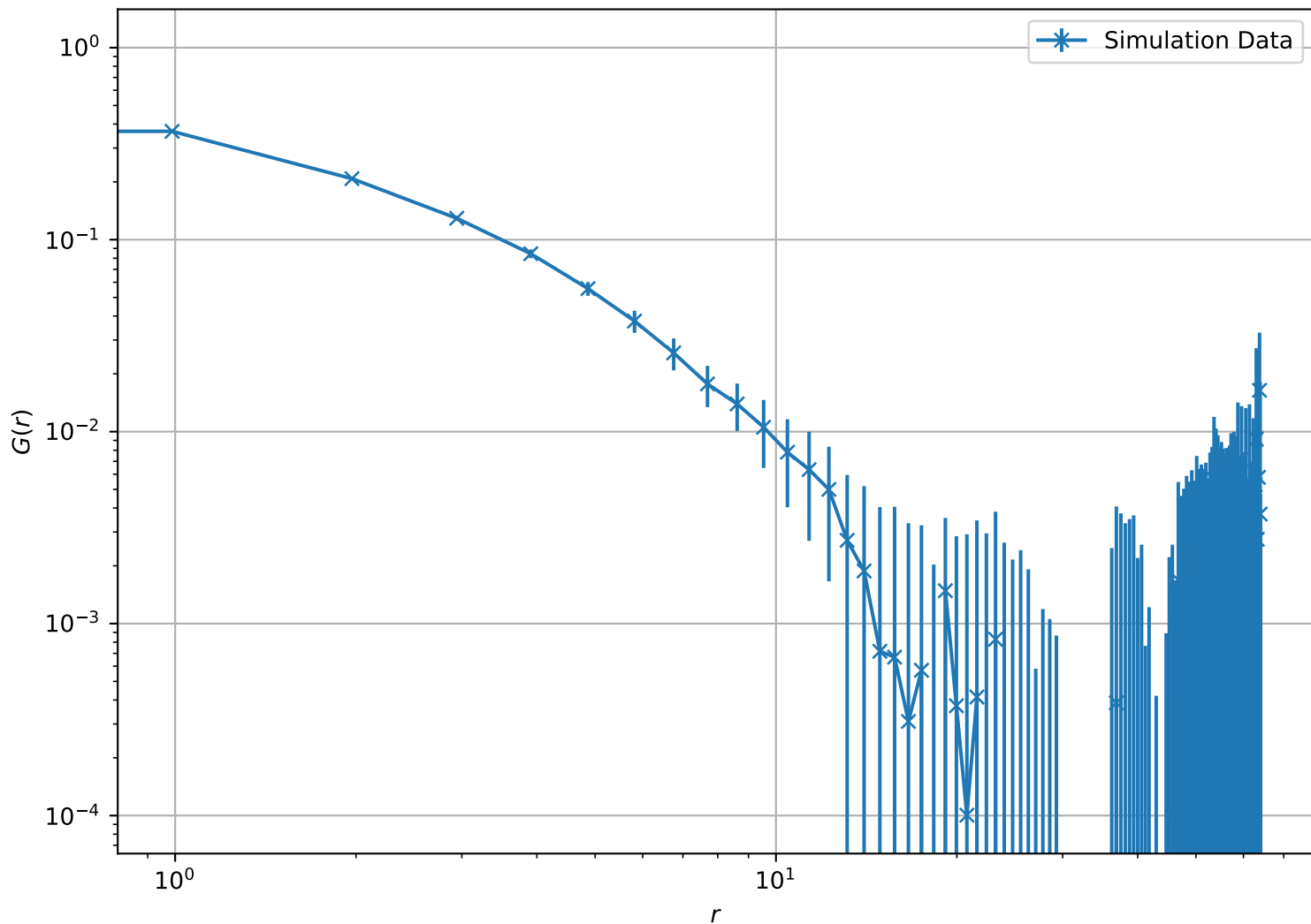
Correlation Function at T = 2.00e + 00 , L = 64 (Log-Log Scale)
