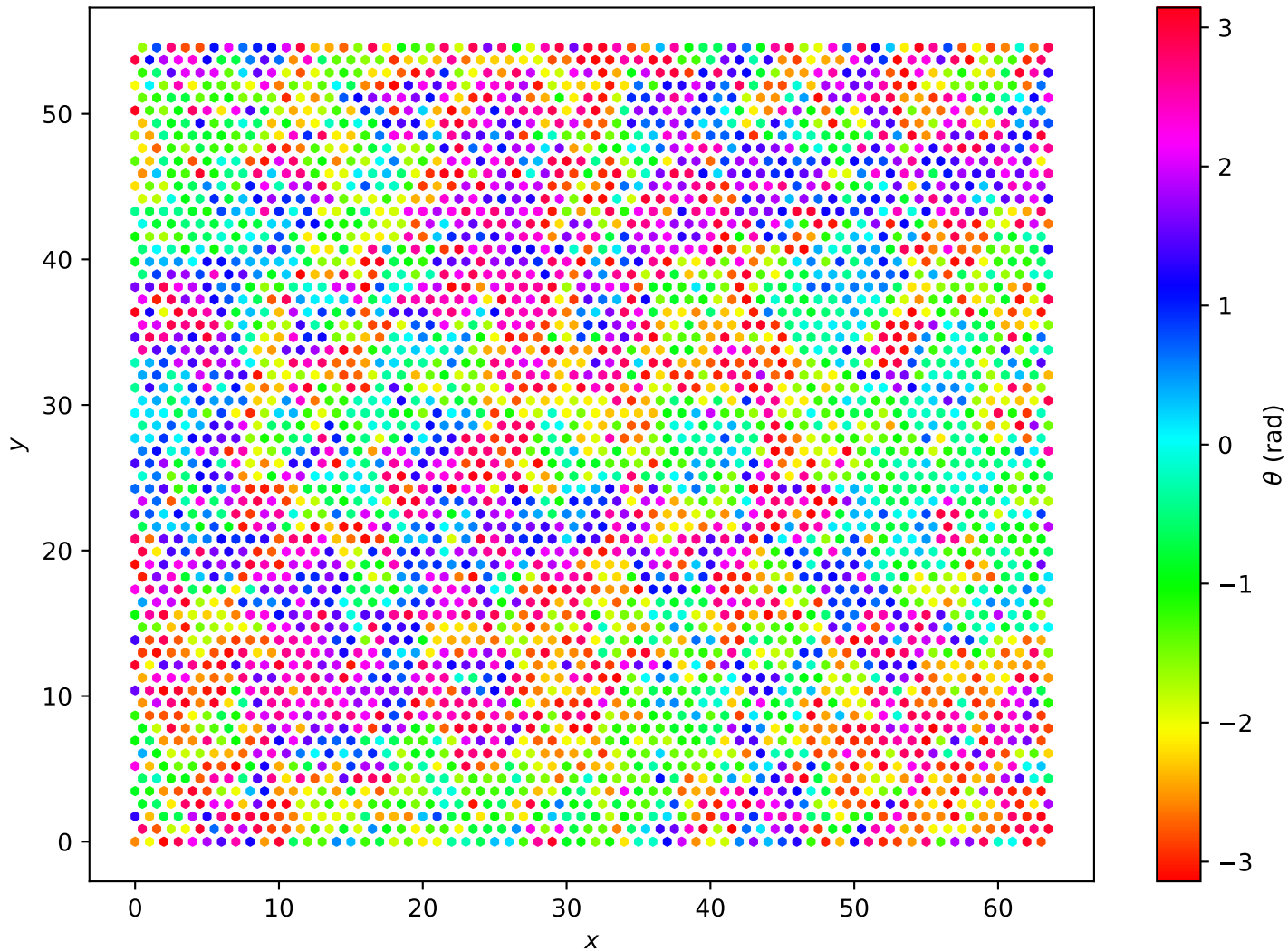
Hexagonal Lattice L=64 , T = 2.00e + 00
