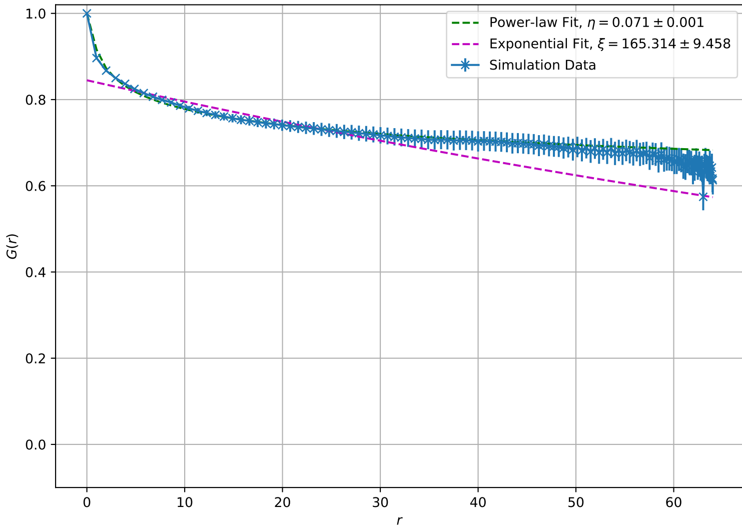
Correlation Function at T = 5.00e - 01 , L = 64
