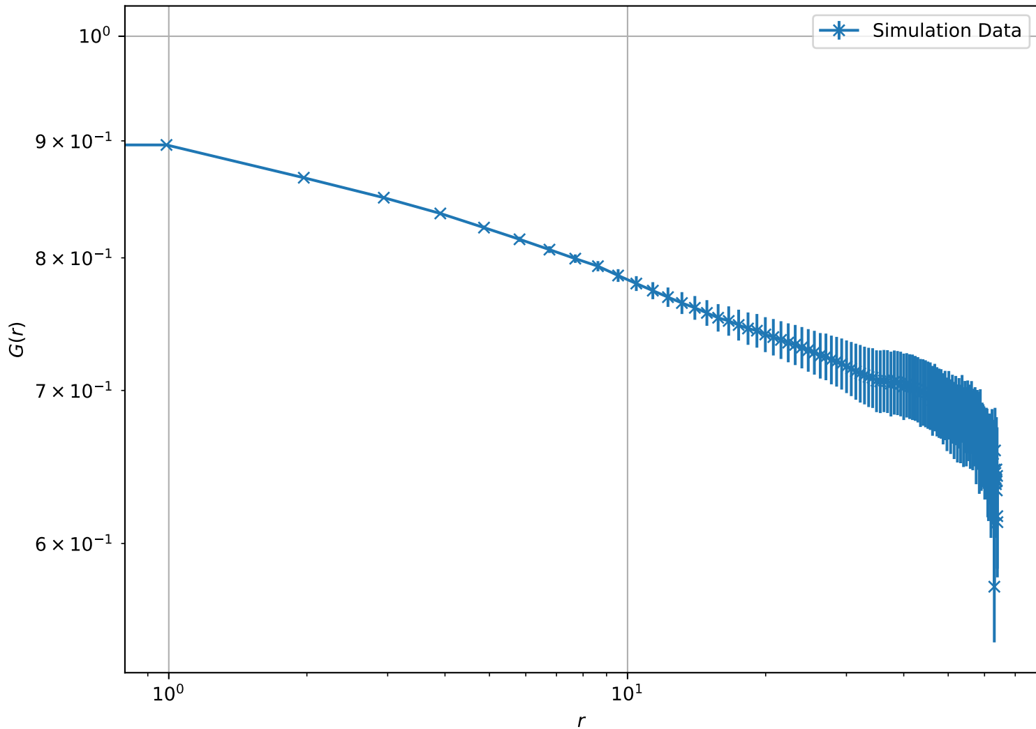
Correlation Function at T = 5.00e - 01 , L = 64 (Log-Log Scale)
