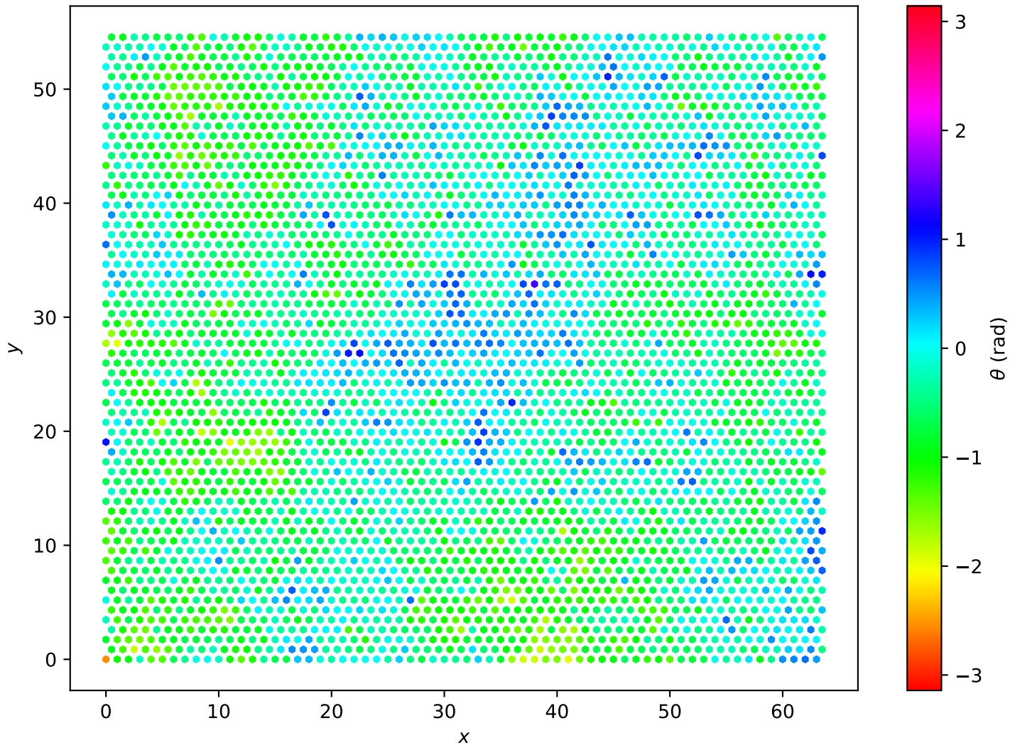
Hexagonal Lattice L=64 , T = 5.00e - 01
