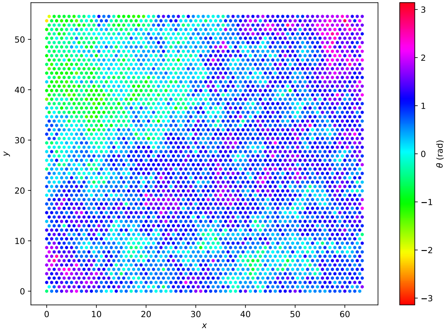
Hexagonal Lattice L=64 , T = 6.00e - 01
