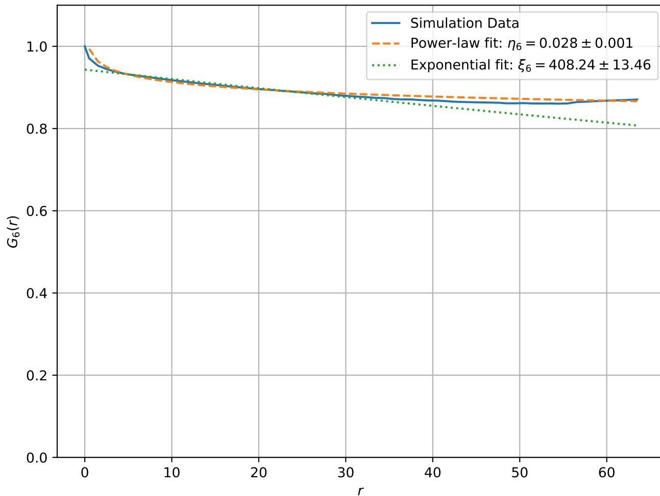
Correlation Function at T = 1.00e - 01 , L = 128
