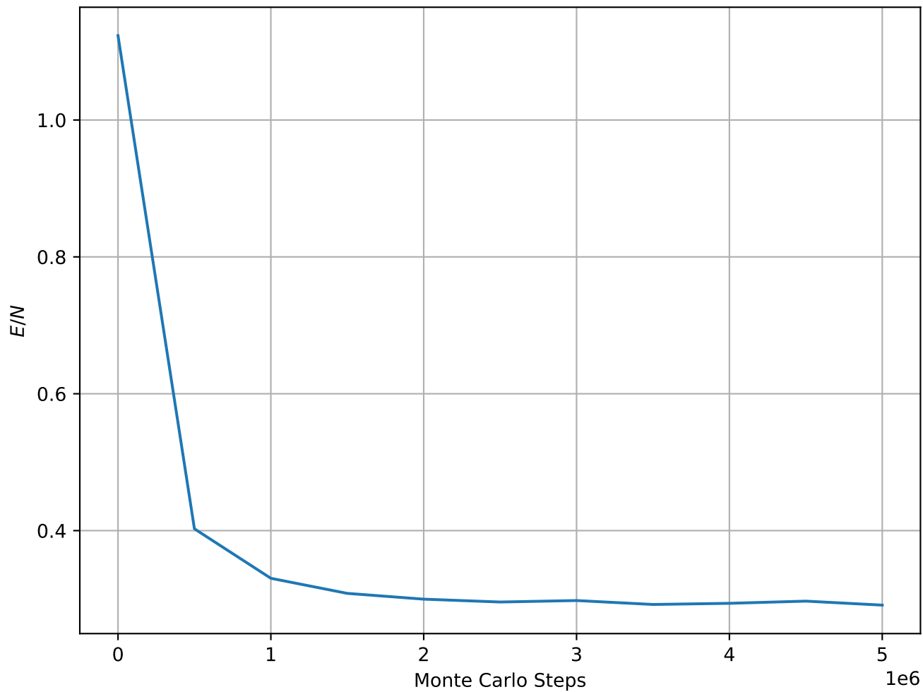
Energy per Spin at T = 1.00e - 01 , L = 128
