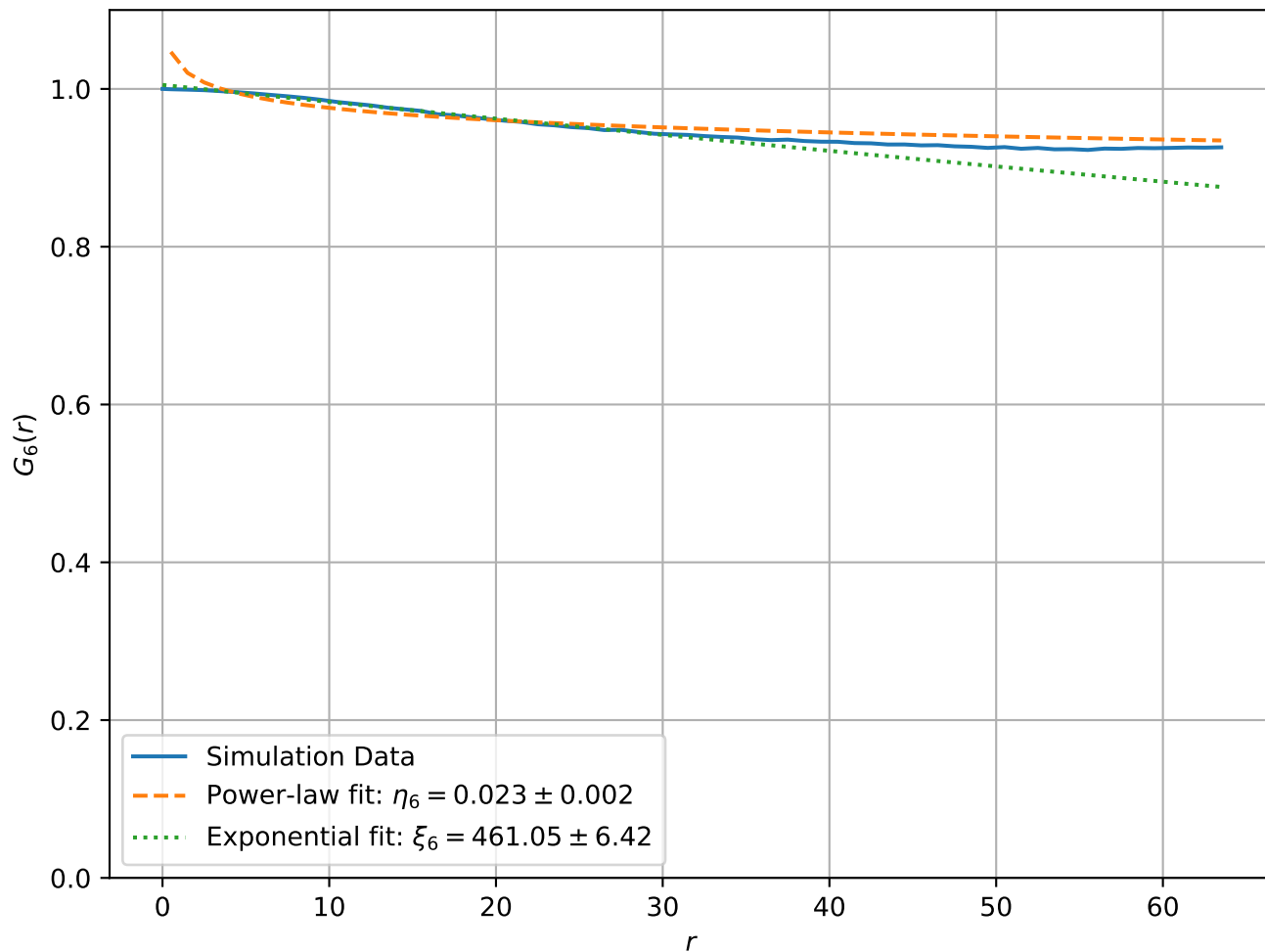
Correlation Function at T = 1.00e - 02 , L = 128
