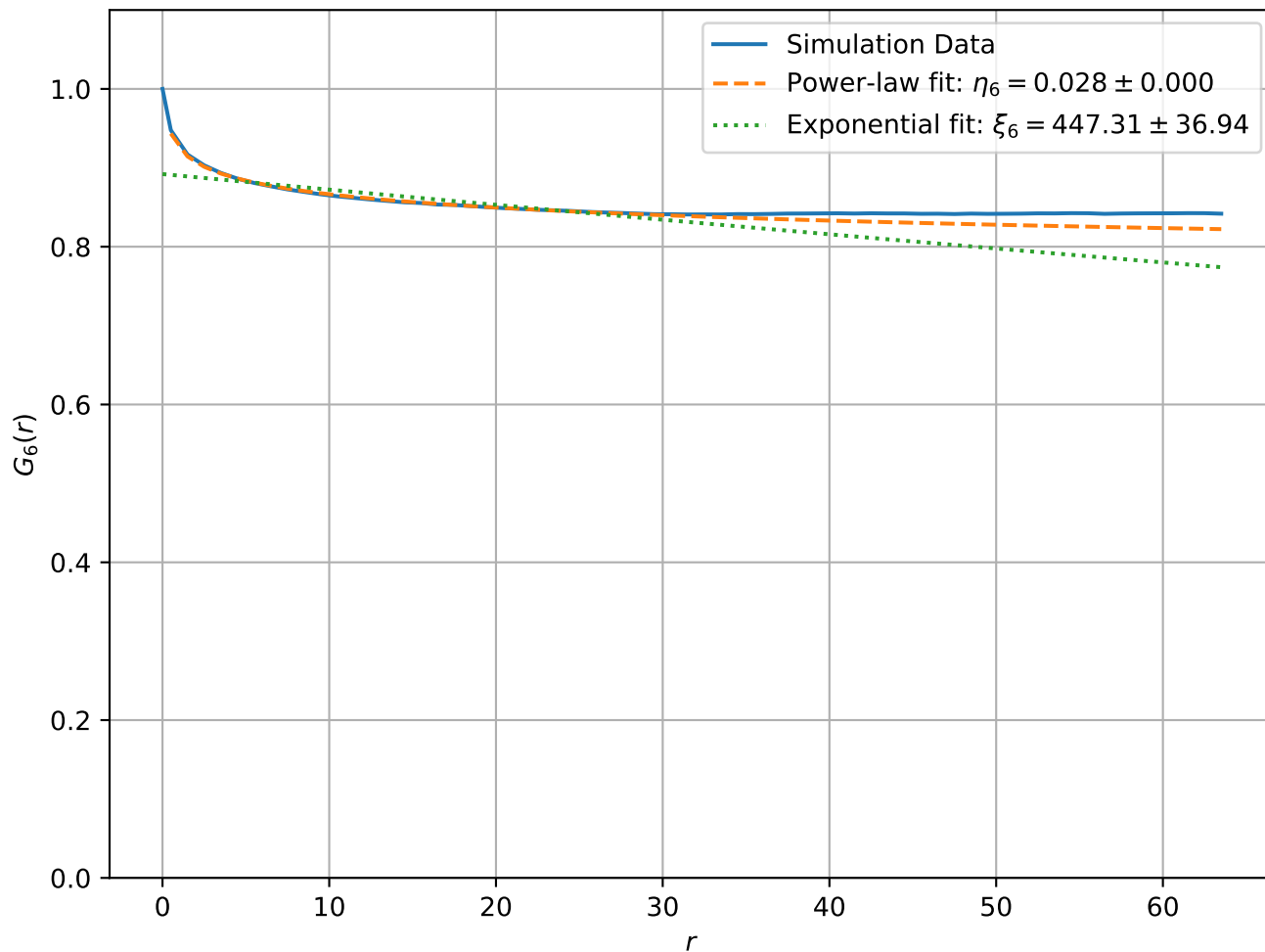
Correlation Function at T = 1.20e - 01 , L = 128
