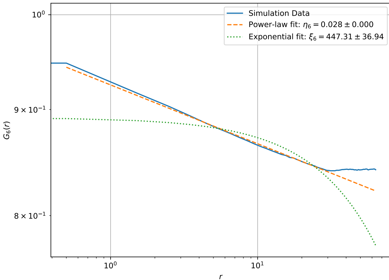
Correlation Function at T = 1.20e - 01 , L = 128 (Log-Log Scale)
