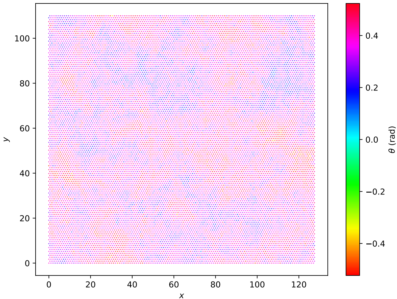
Hexagonal Lattice L=128 , T = 1.20e - 01
