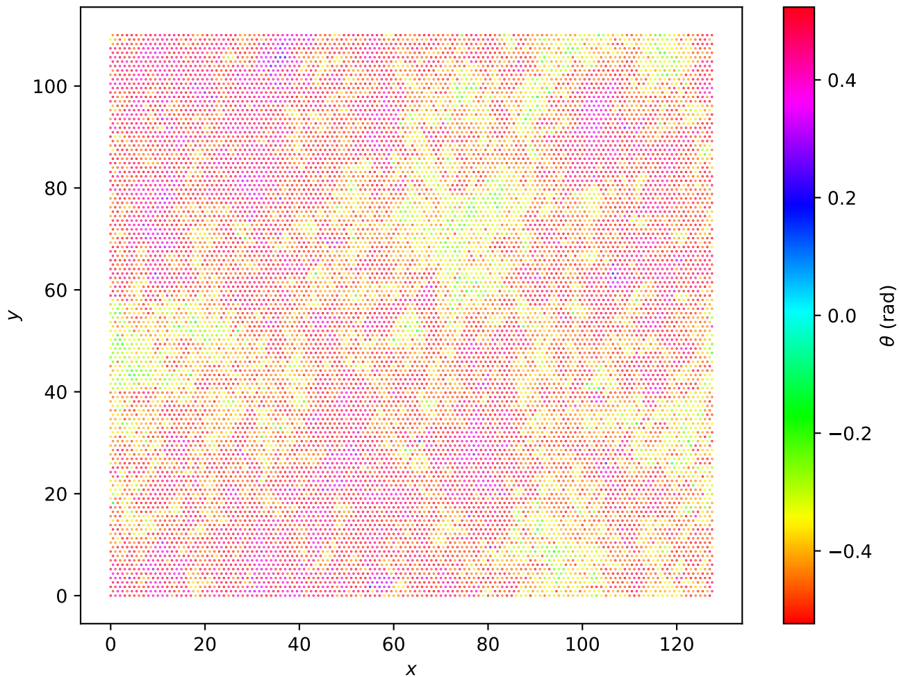
Hexagonal Lattice L=128 , T = 1.50e - 01
