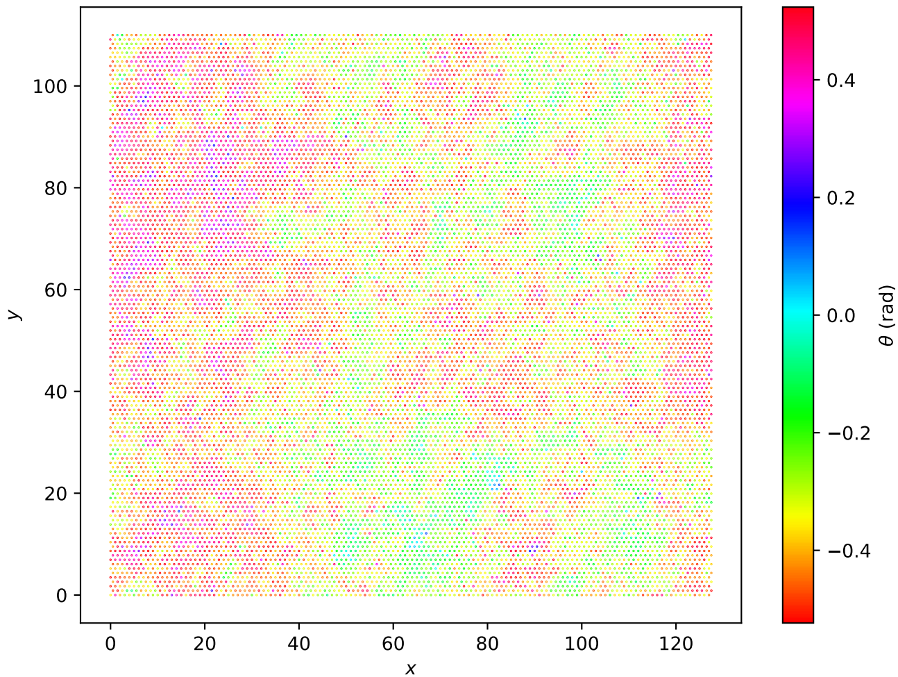
Hexagonal Lattice L=128 , T = 1.70e - 01
