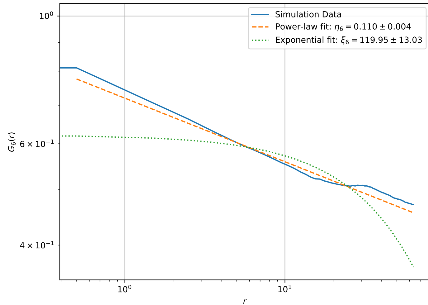
Correlation Function at T = 1.80e - 01 , L = 128 (Log-Log Scale)
