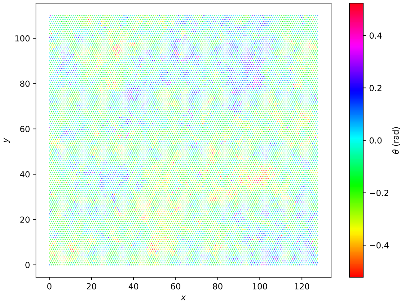
Hexagonal Lattice L=128 , T = 1.80e - 01
