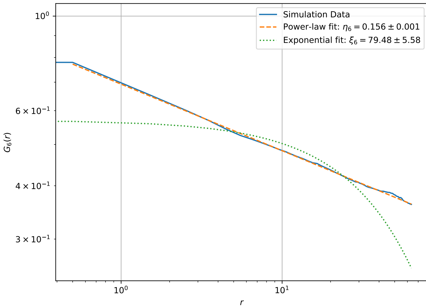
Correlation Function at T = 1.90e - 01 , L = 128 (Log-Log Scale)
