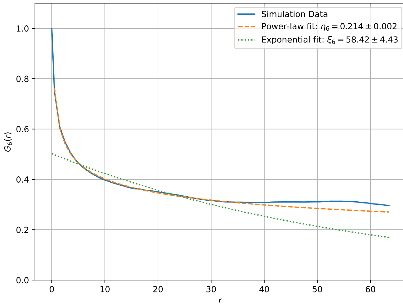
Correlation Function at T = 1.95e - 01, L = 128
