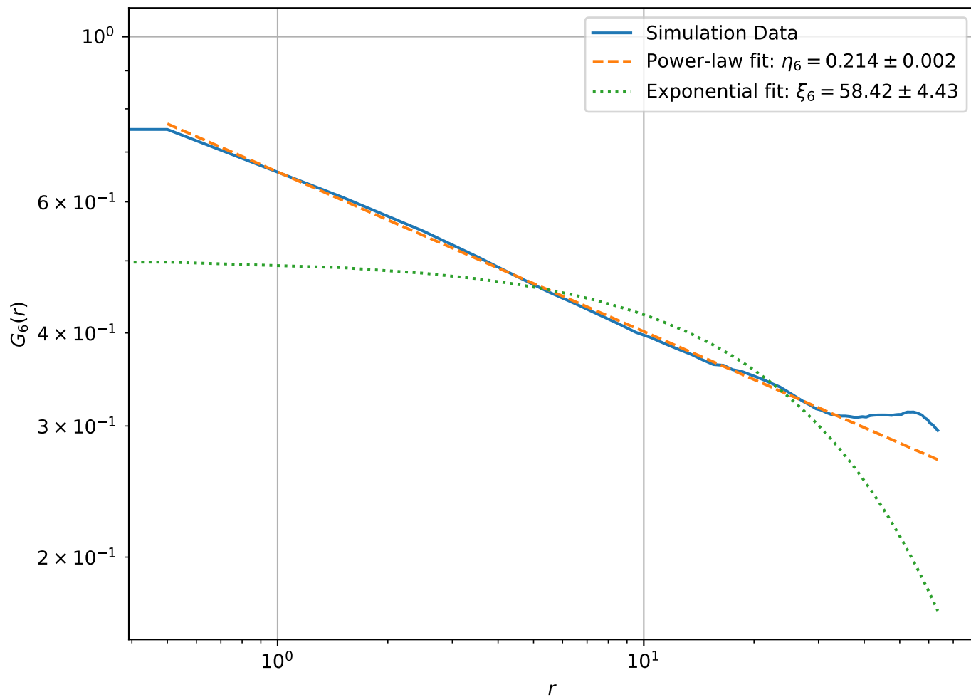
Correlation Function at T = 1.95e - 01 , L = 128 (Log-Log Scale)
