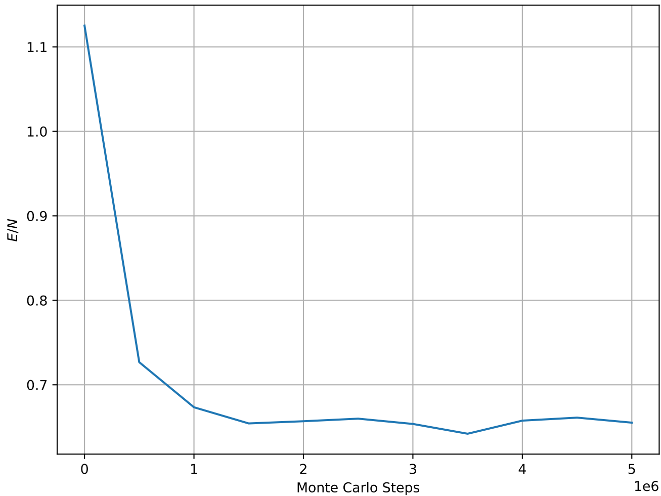
Energy per Spin at T = 1.95e - 01 , L = 128
