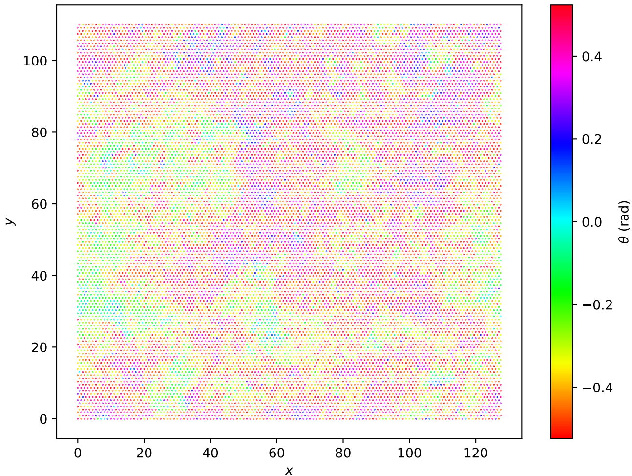
Hexagonal Lattice L=128 , T = 1.95e - 01
