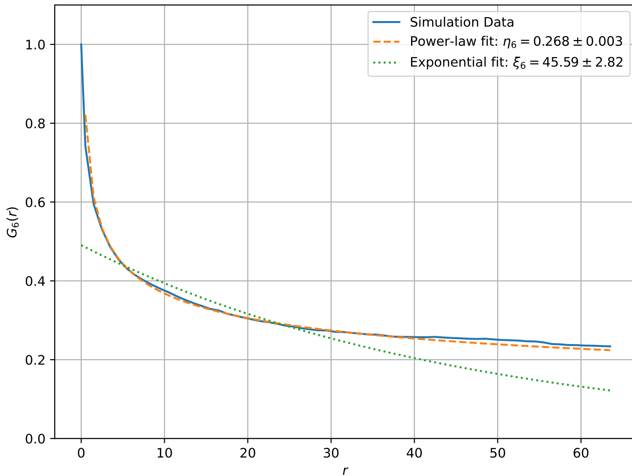
Correlation Function at T = 1.96e - 01, L = 128
