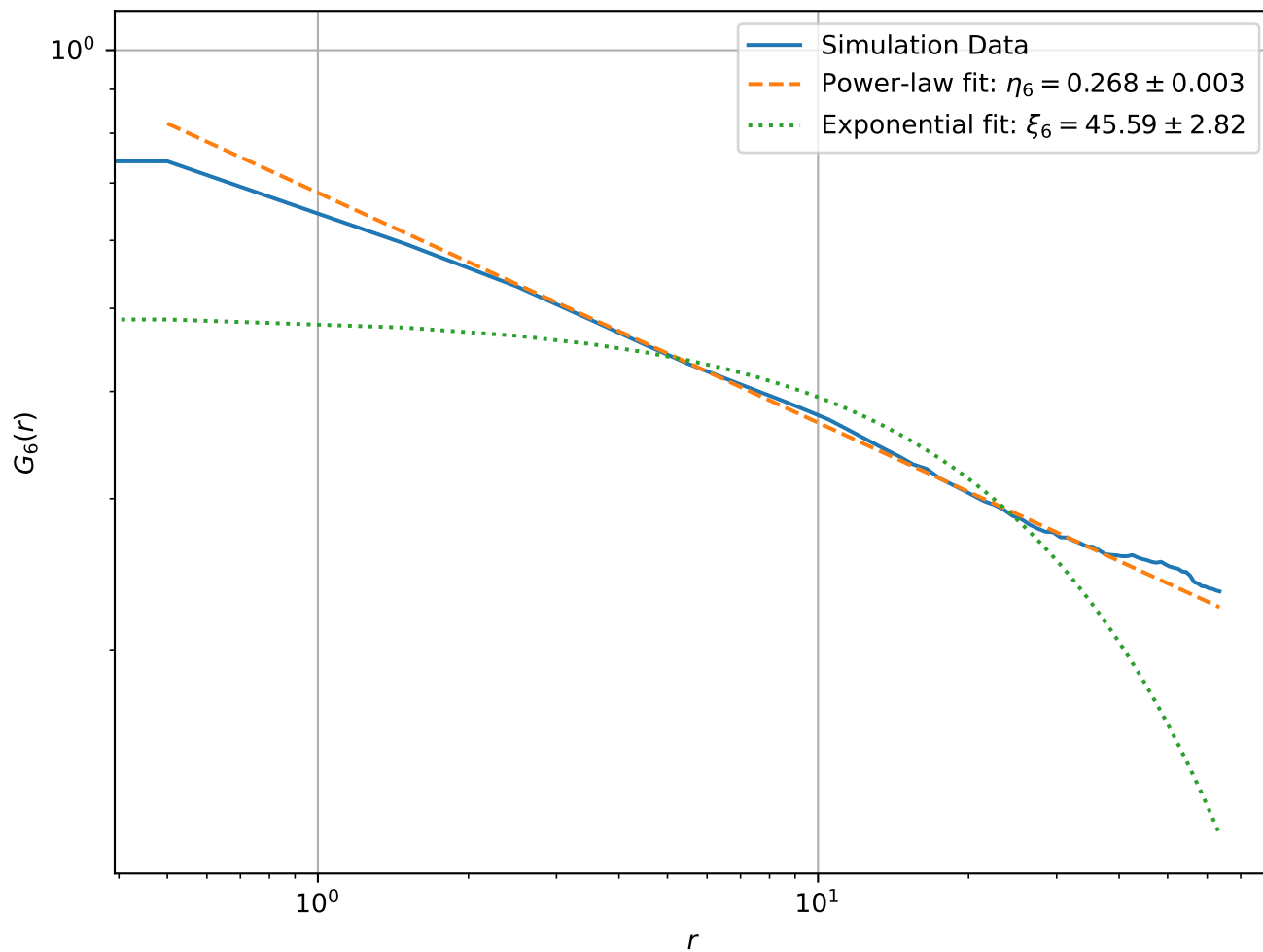
Correlation Function at T = 1.96e - 01 , L = 128 (Log-Log Scale)
