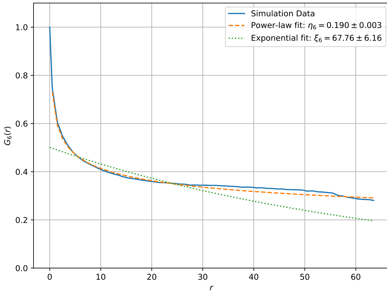
Correlation Function at T = 1.97e - 01, L = 128
