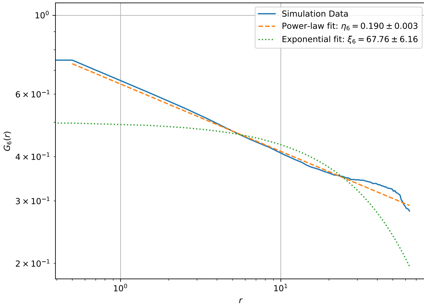
Correlation Function at T = 1.97e - 01 , L = 128 (Log-Log Scale)
