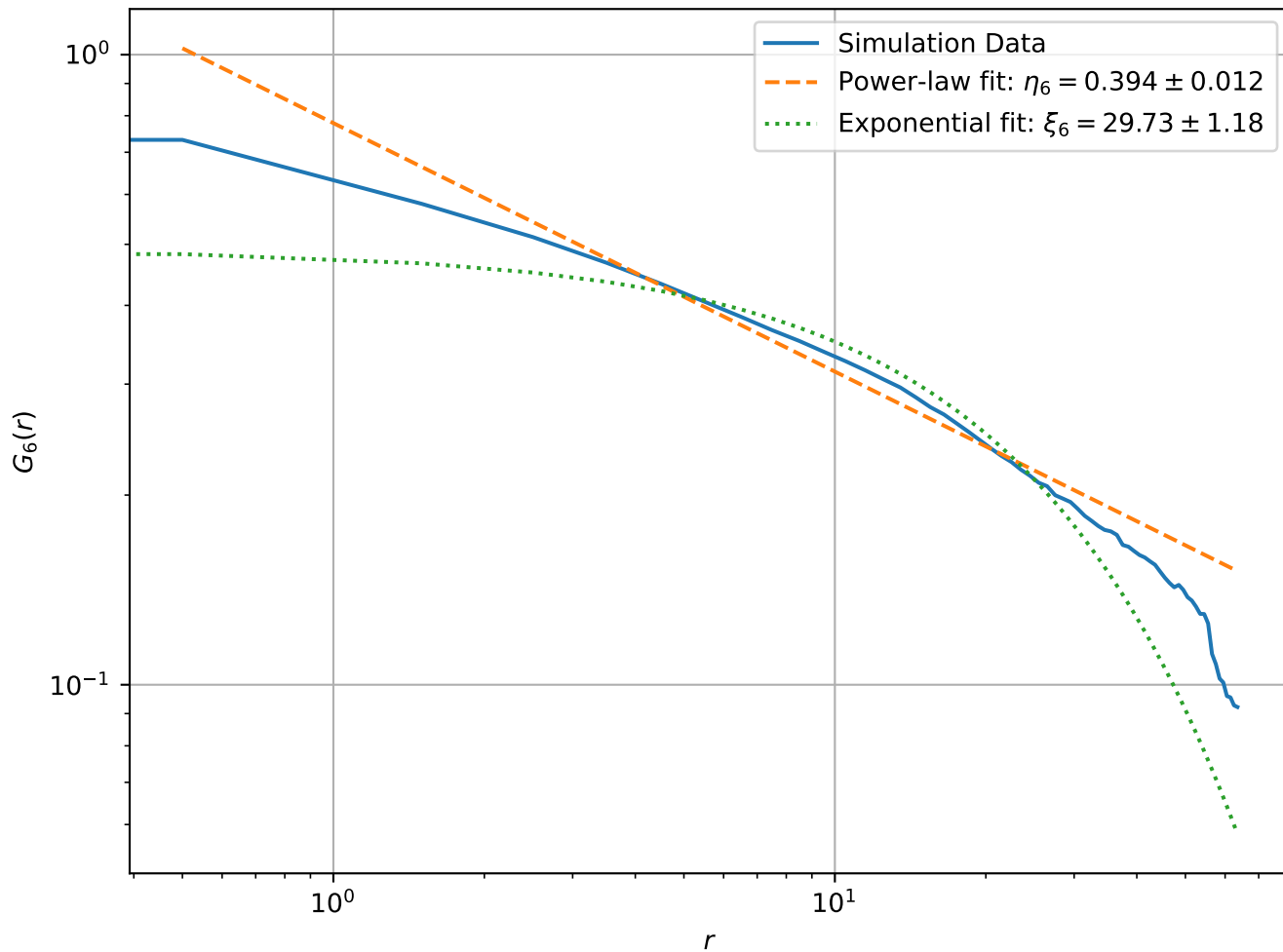
Correlation Function at T = 1.98e - 01 , L = 128 (Log-Log Scale)
