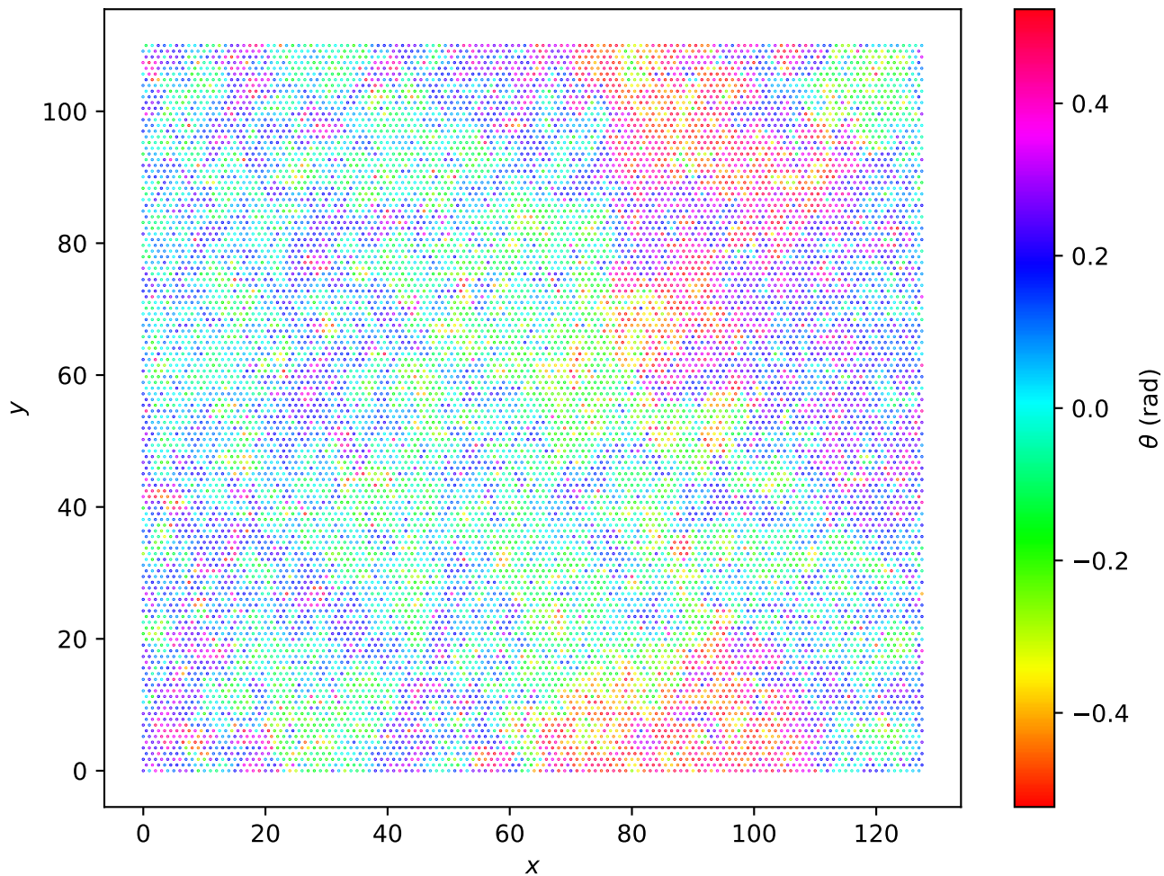
Hexagonal Lattice L=128 , T = 1.98e - 01
