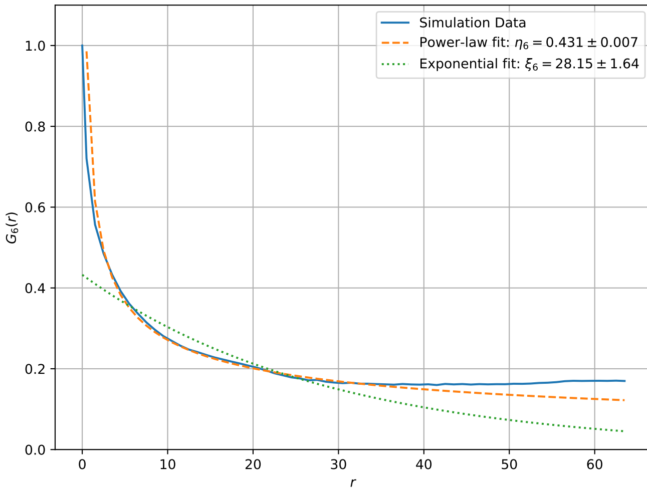
Correlation Function at T = 1.99e - 01 , L = 128
