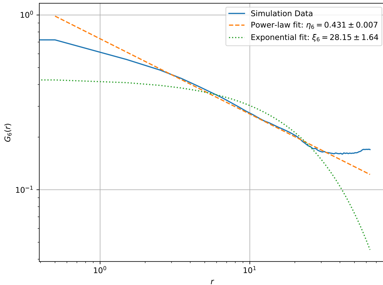
Correlation Function at T = 1.99e - 01 , L = 128 (Log-Log Scale)
