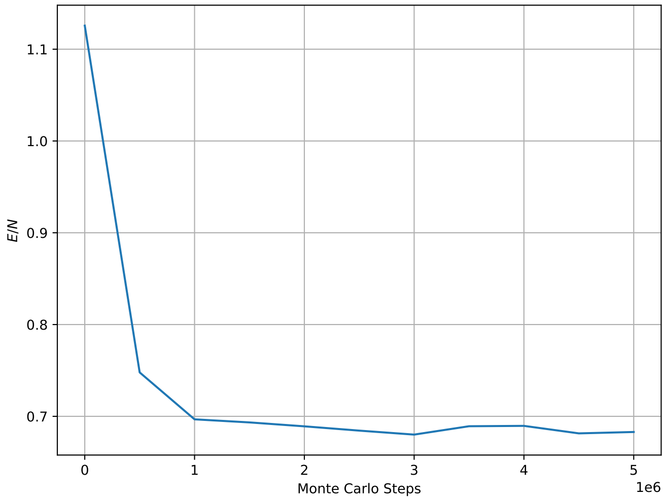
Energy per Spin at T = 1.99e - 01 , L = 128
