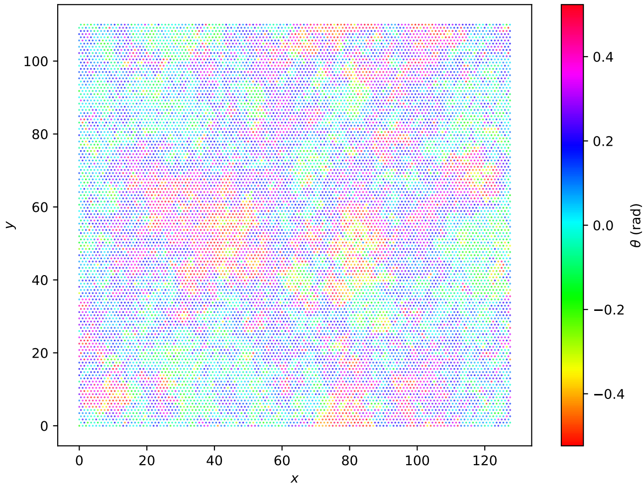
Hexagonal Lattice L=128 , T = 1.99e - 01
